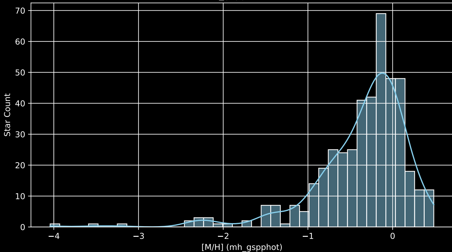
APOGEE DR17 Field: [094+00 [M/H] (mh_gspphot) (n= 439)
