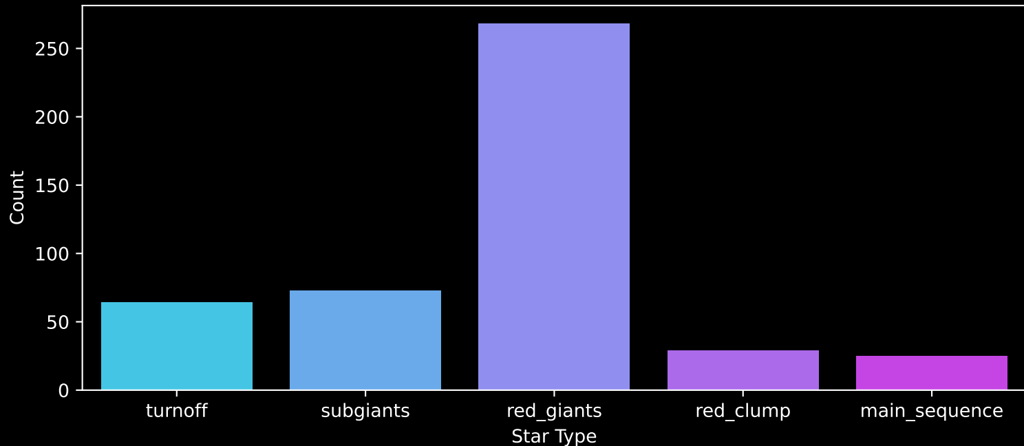
APOGEE DR17 Field: [094+00] Count plot of Star Type
