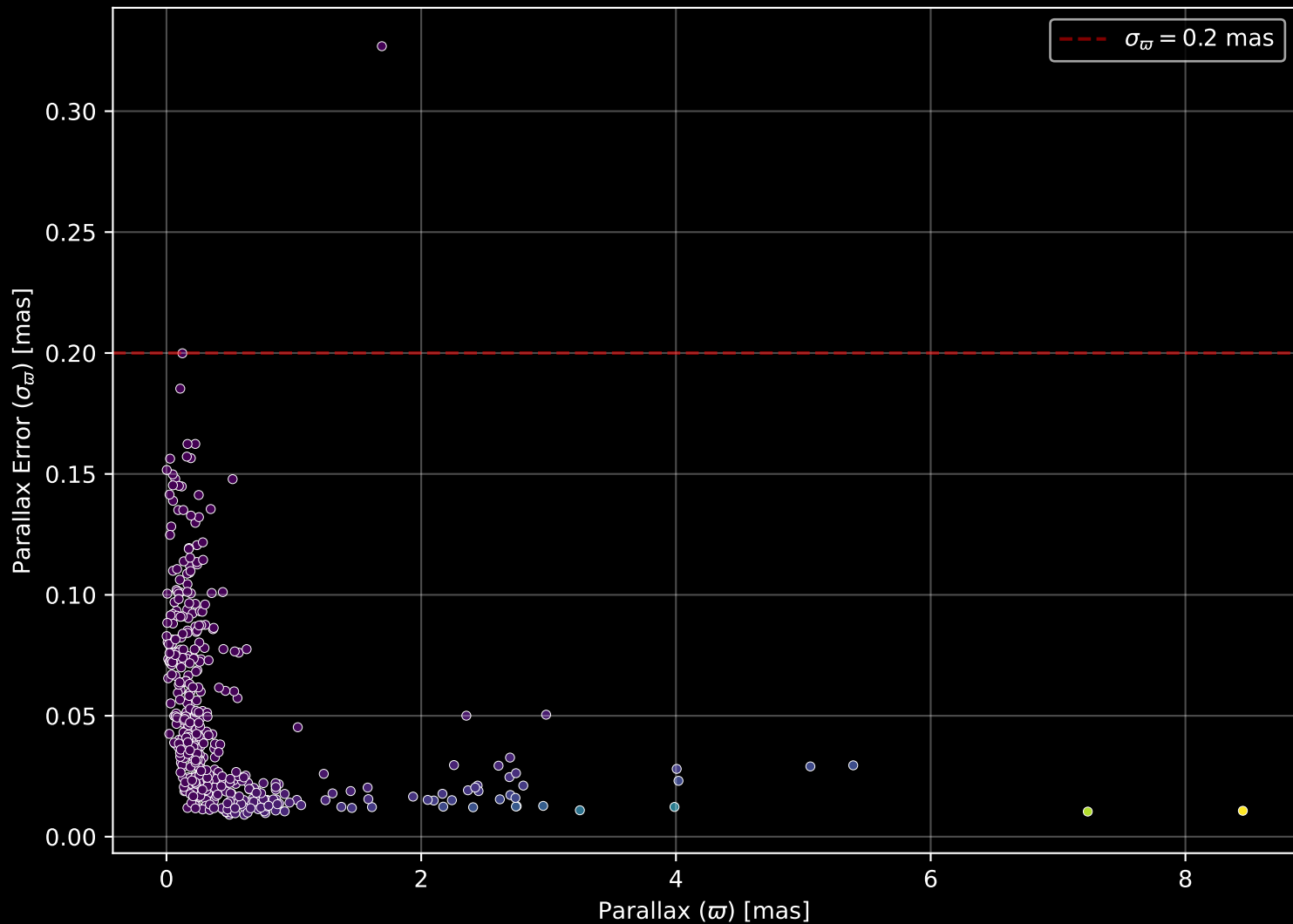
APOGEE DR17 Field: [094+00] Parallax Quality (n= 459)
