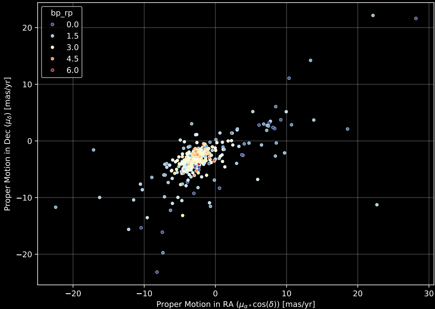
APOGEE DR17 Field: [094+00] Proper Motion Diagram (n= 459)
