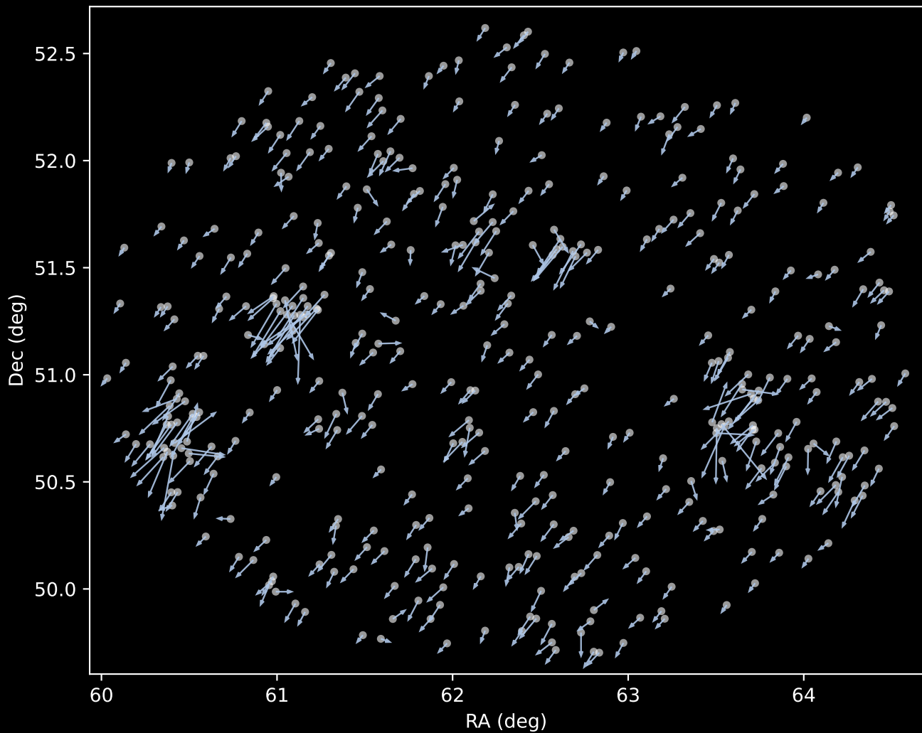
APOGEE DR17 Cluster 1 Proper Motion Vectors (n=419)
