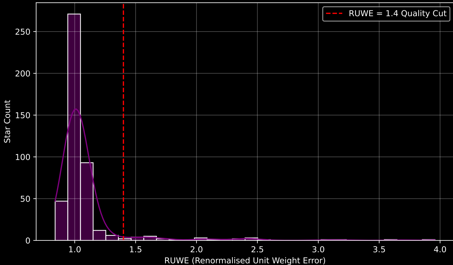
GAPOGEE DR17 Field [094+00] RUWE Distribution (n= 457)
